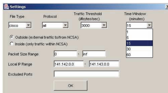
Figure 6. Setting Dialog
